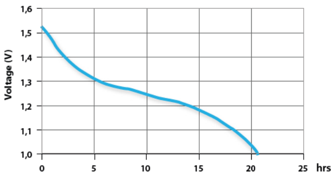
Remote Control 15s/m 8h/d 24 ohm end 1,0V
